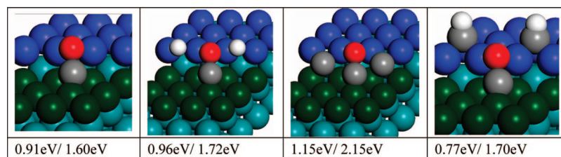
Figure 6. Calculated reaction barriers and the transition state snapshots of CO dissociation with and without coadsorbates. The reaction barriers beneath the figures are for Ru and Rh, respectively.
