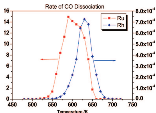
Figure 7. Calculated rate of CO dissociation on Ru and Rh at various temperatures
